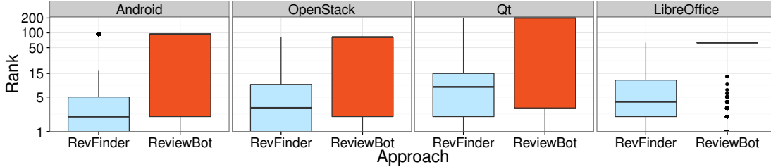
Fig. 4: A rank distribution of the first correct code-reviewers recommended by RevFinder and ReviewBot. The results show that RevFinder provide a better ranking of recommended code-reviewers.
