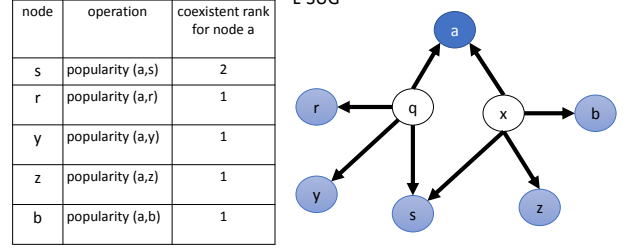
Fig. 4. Example of the coexistence operation. For the L-SUG P' , for a node a , the coexistence rank allows to determine popularity in relation to node a . In this example node s has the highest coexistence rank.
