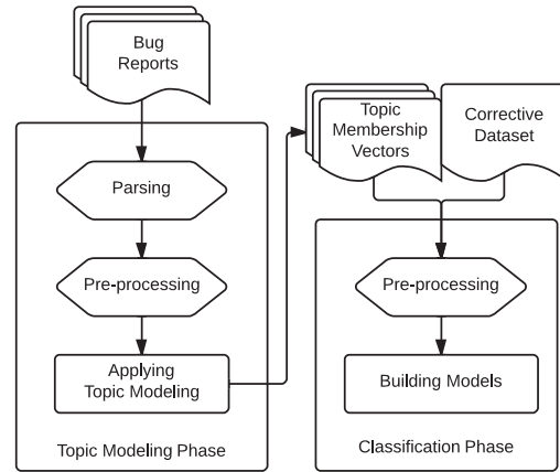
Figure 1. Overview of our automatic classification model building process
